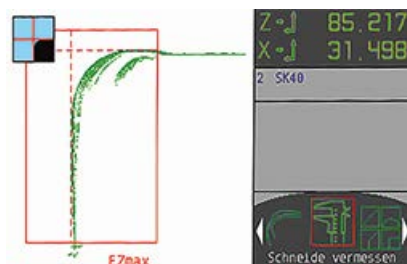
EZmax – Software function for determining and measuring the tool contour
