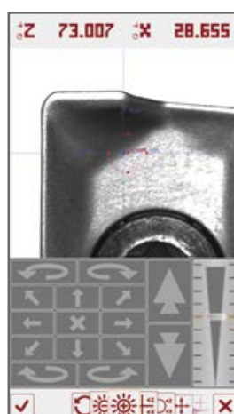
Tool cutting edges in incident light with 20x zoom to inspect cutting edges for wear and tool breakage
